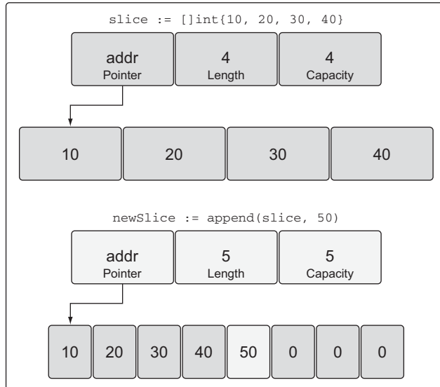
Figure 4.15 The new underlying array after the append operation
