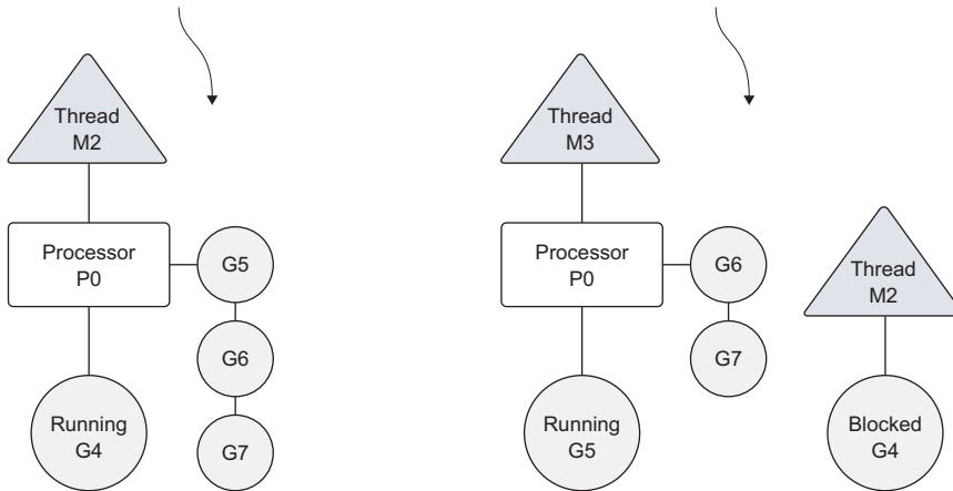
Figure 6.2 How the Go scheduler manages goroutines
